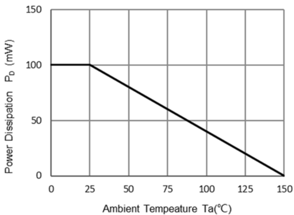
Fig 5: P_D-Ta Curve
