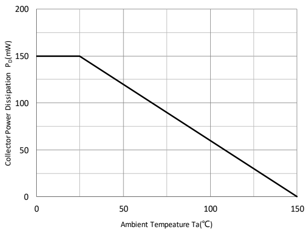
Fig 5: P_D-Ta Curve
