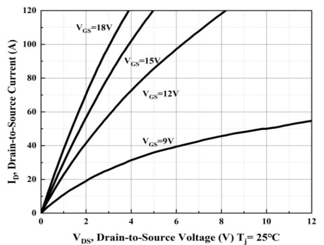
Figure2. Output Characteristics T j = 25℃
