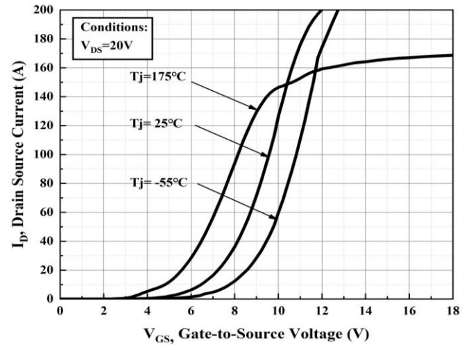
Figure 4. Transfer Characteristics for Various Junction Temperature
