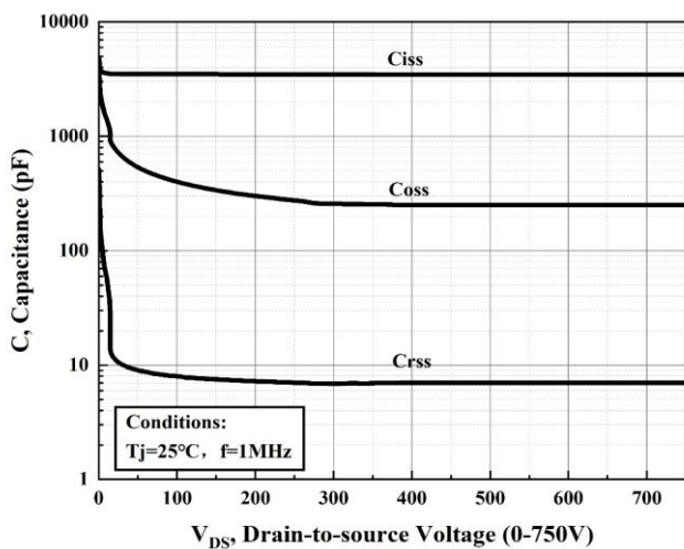
Figure 13. Capacitances vs. Drain Source Voltage (0-750V)
