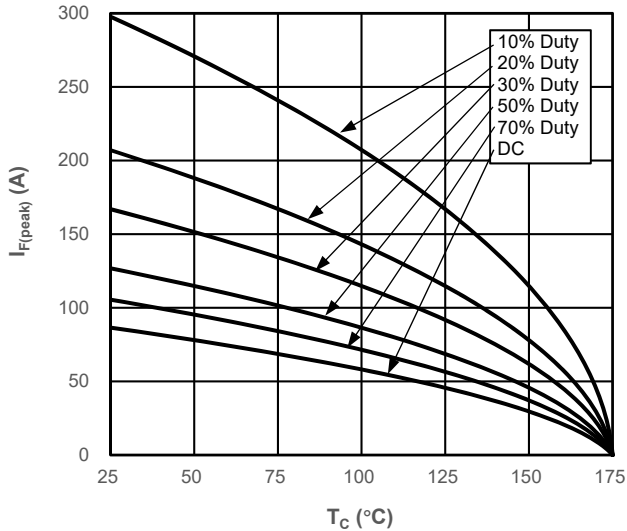
Fig3. Current Derating
