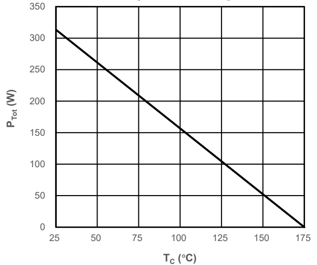
Fig4. Power Derating
