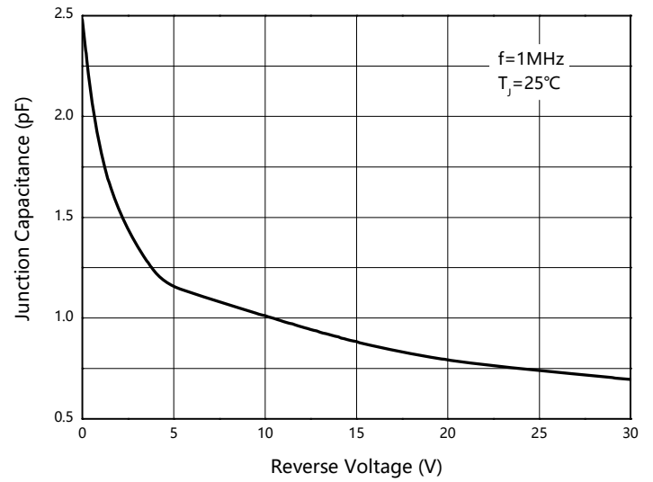
Fig.2: Capacitance Characteristics
