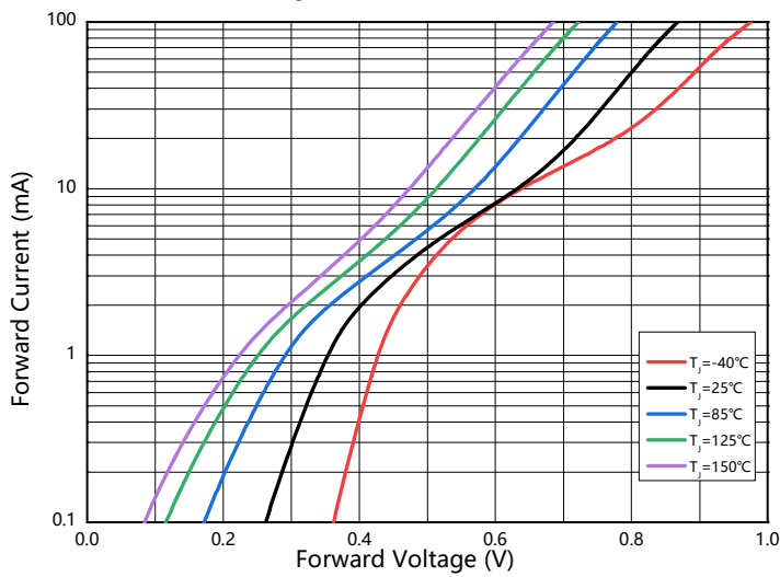
Fig.3: Forward Characteristics
