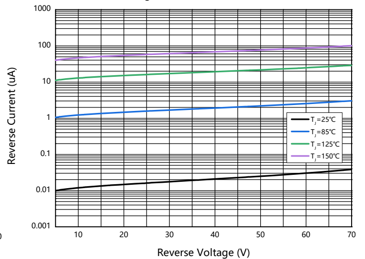
Fig.4: Reverse Characteristics
