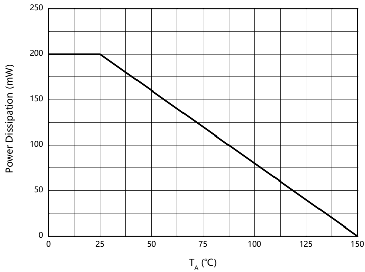
Fig.1: P_D - T_A
