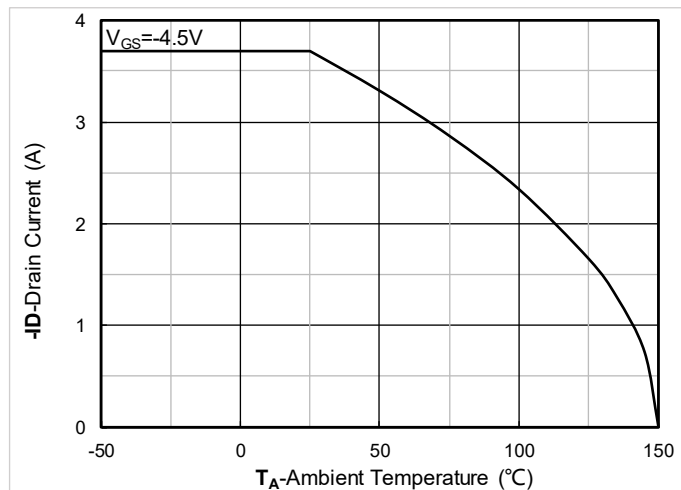
Figure8. Maximum Continuous Drain Current vs Ambient Temperature
