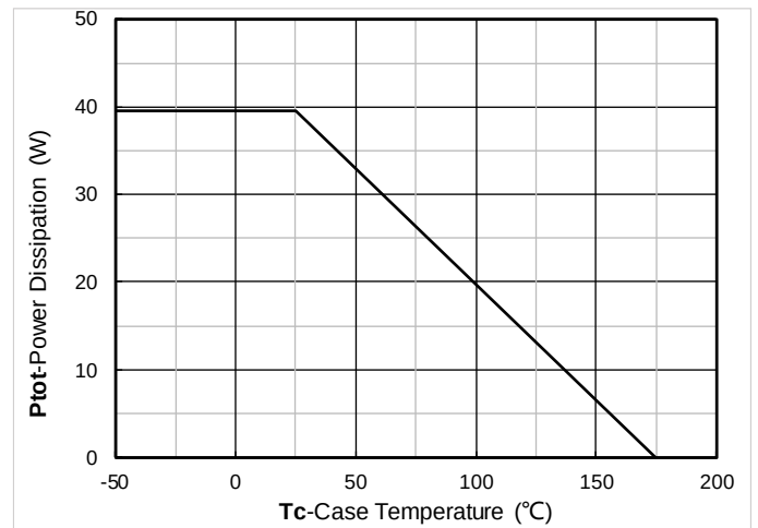
Figure 12. Power dissipation
