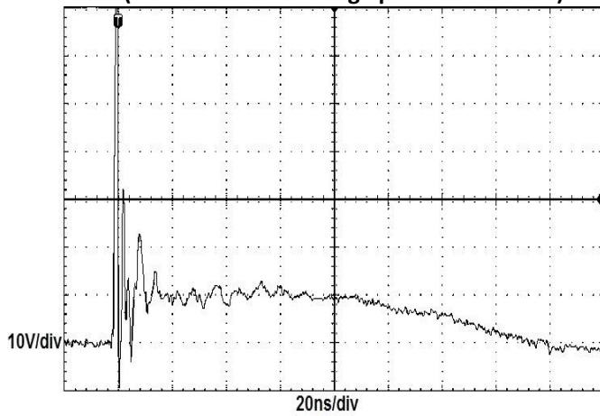
TLP Measurement
